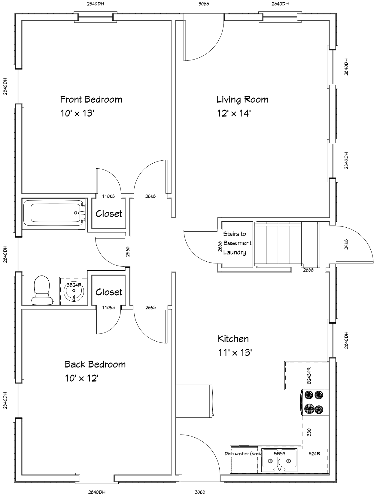
1st Floor LIVING AREA 840 SQ FT
