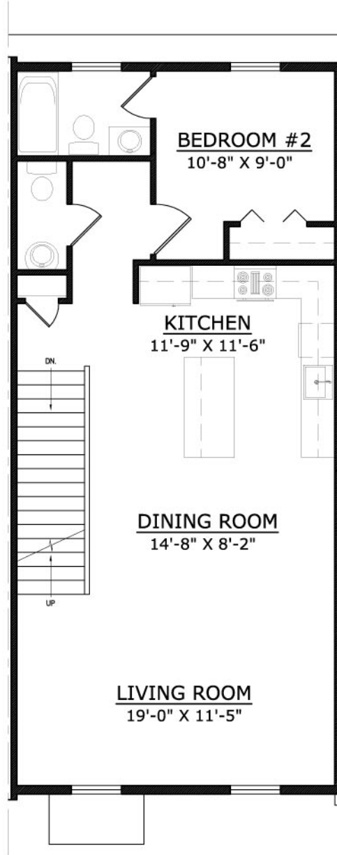
SECOND FLOOR PLAN APPROX. 835 S.F. PER UNIT
