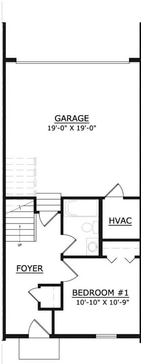
FIRST FLOOR PLAN APPROX. 377 S.F. PER UNIT
