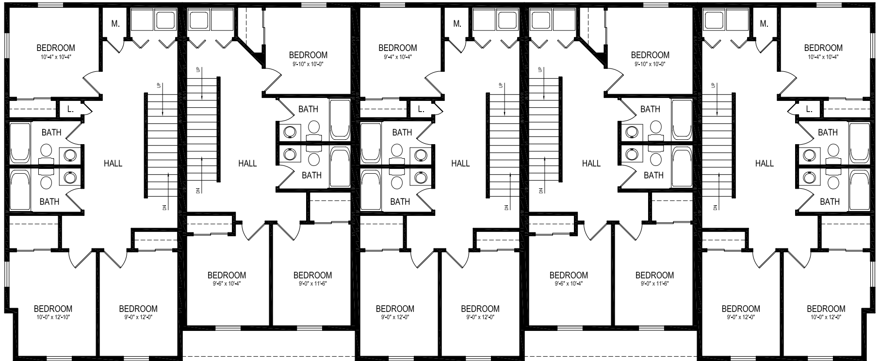
○ 2nd FLOOR PLANS N.T.S.
