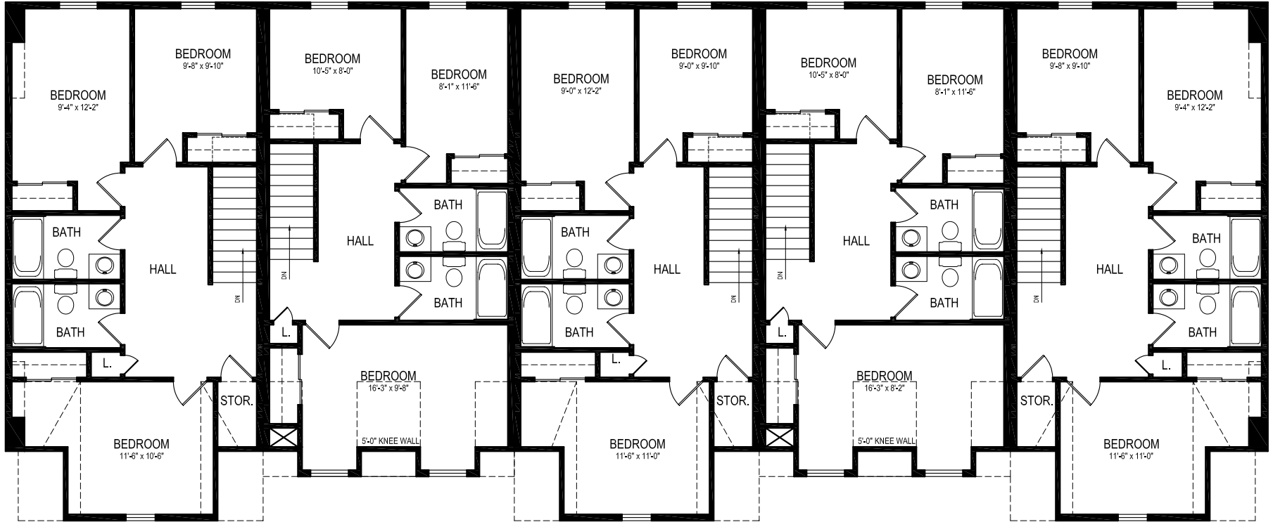
3rd FLOOR PLANS N.T.S.
