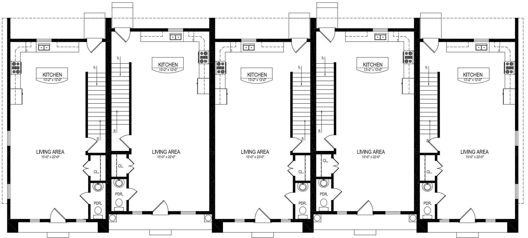
○ 1st FLOOR PLANS N.T.S.
